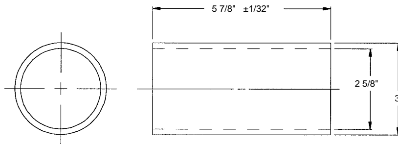
Part No. 38127 For 2 1/2 in. or 2 9/16 in. diameter rollers
