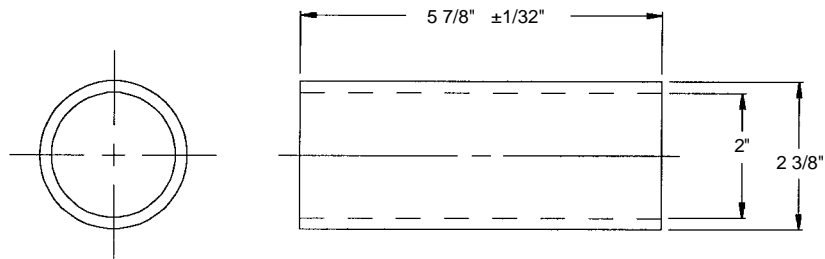
Part No. 38126 For 1.9 in. diameter roller
