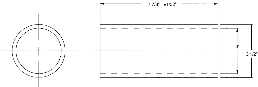
Part No. 38128 For 2 7/8 in. diameter roller
