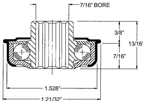
Bearing No. 102031
