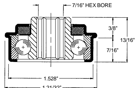
Bearing No. 102072
