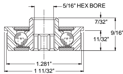
Bearing No. 102274
