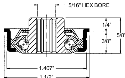
Bearing No. 102175
