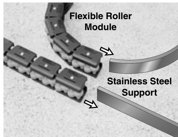
Modules slide onto 40mm x 8 mm flat bars or the "M". Minimum radius for a curved section is 10 in. (beads outside) and 12 in. (beads inside).
