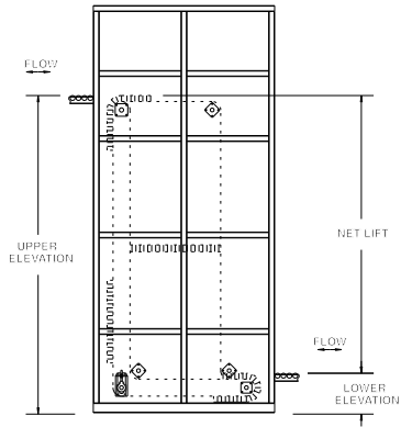
CVC-Z SIDE VIEW
