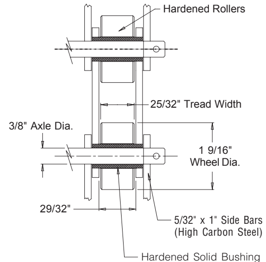
Wheel Cross Section
